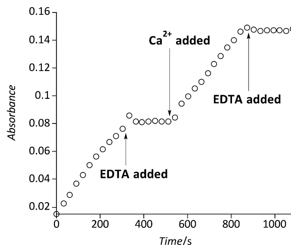
Figure 1. Allosteric regulation of AlleyCat7. Experimental conditions: initial concentrations: 130 nM protein, 100 mM NaCl, 20 mM HEPES buffer, pH 7.0, 0.1 mM CaCl 2 , 0.1 mM substrate. At 300 s EDTA (ethylenediaminetetraacetic acid) was added to the final concentration of 0.2 mM, followed by addition of CaCl 2 at 540 s to the final concentration of 0.3 mM and, again, EDTA at 840 s to the final concentration of 0.5 mM.
